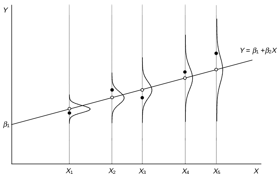
Figure 8.2 Heteroscedasticity
