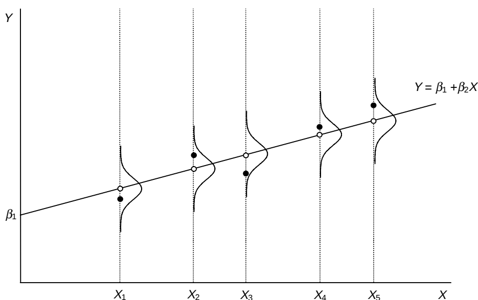
Figure 8.1 Homoscedasticity
